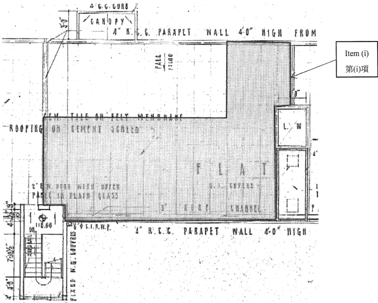
FLAT B3 ON ROOF FLOOR PLAN B3室天台平面圖
